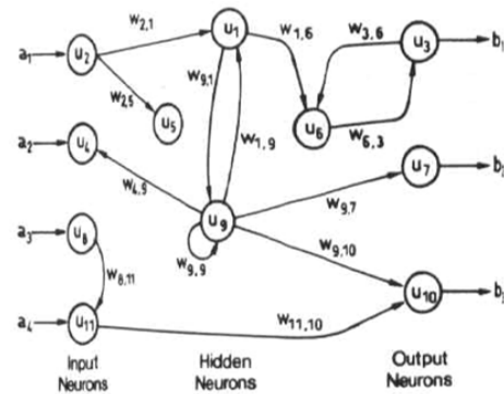
Figure 2.7: Recurrent network. [60]
